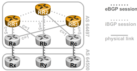
Fig. 4. Topology of experimentation.
